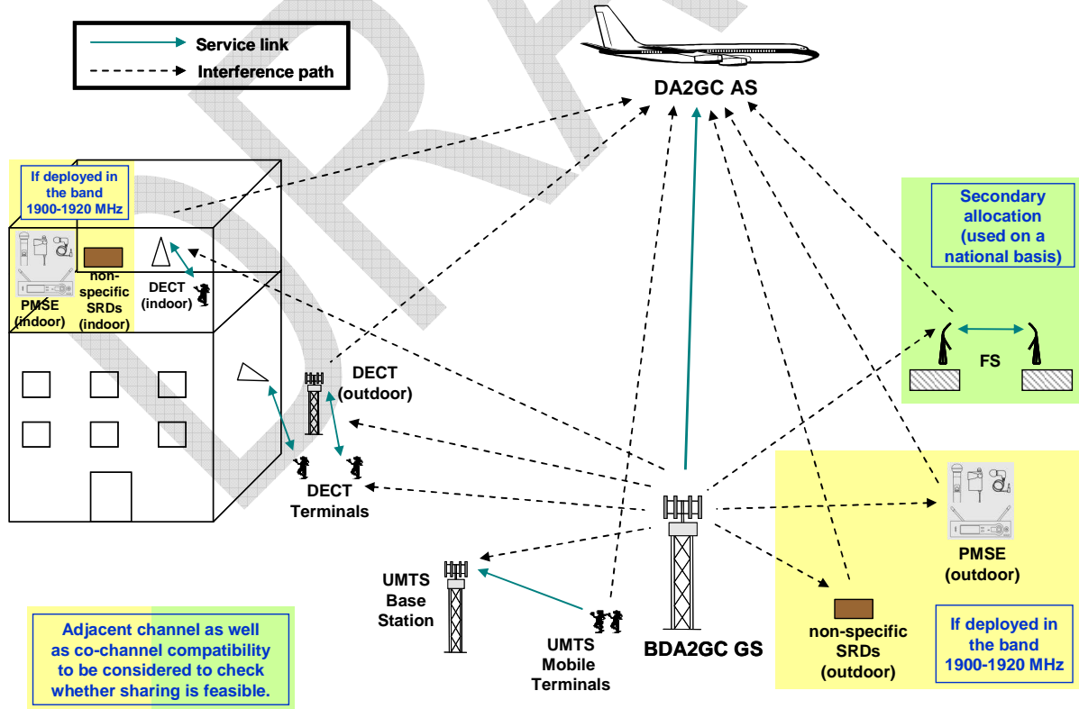
Figure 4: Compatibility/sharing scenarios for BDA2GC FL in the frequency band 1900-1920 MHz
