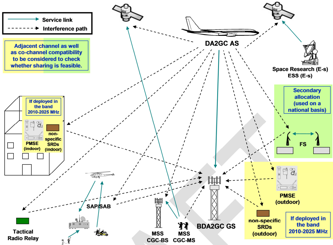
Figure 5: Compatibility/sharing scenarios for DA2GC RL in the frequency band 2010-2025 MHz
