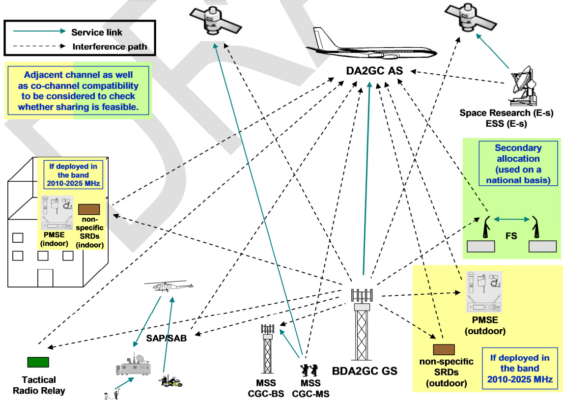
Figure 6: Compatibility/sharing scenarios for DA2GC FL in the frequency band 2010-2025 MHz
