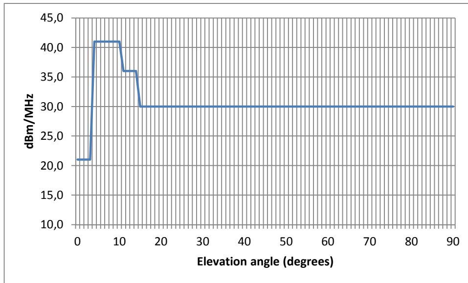
Figure 17: Peak e.i.r.p. mask for the Ground Station according to ETSI TR 103 108 [33]
