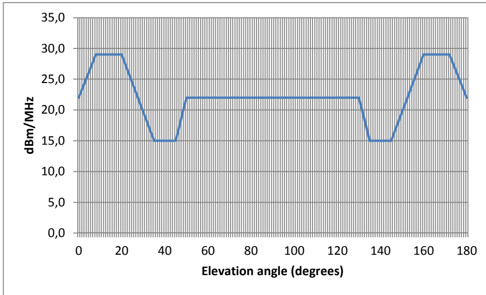
Figure 18: Peak e.i.r.p. mask for Aircraft Station (AS)
