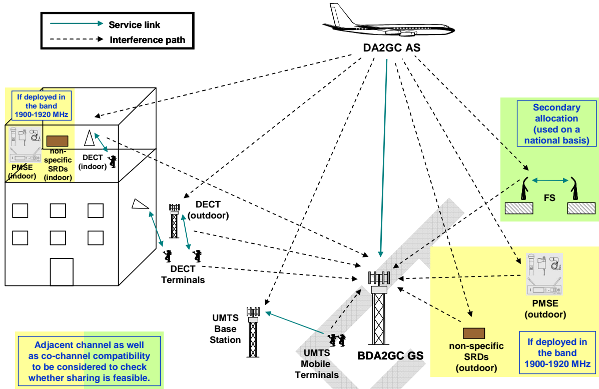
Figure 3: Compatibility/sharing scenarios for BDA2GC RL in the frequency band 1900-1920 MHz
