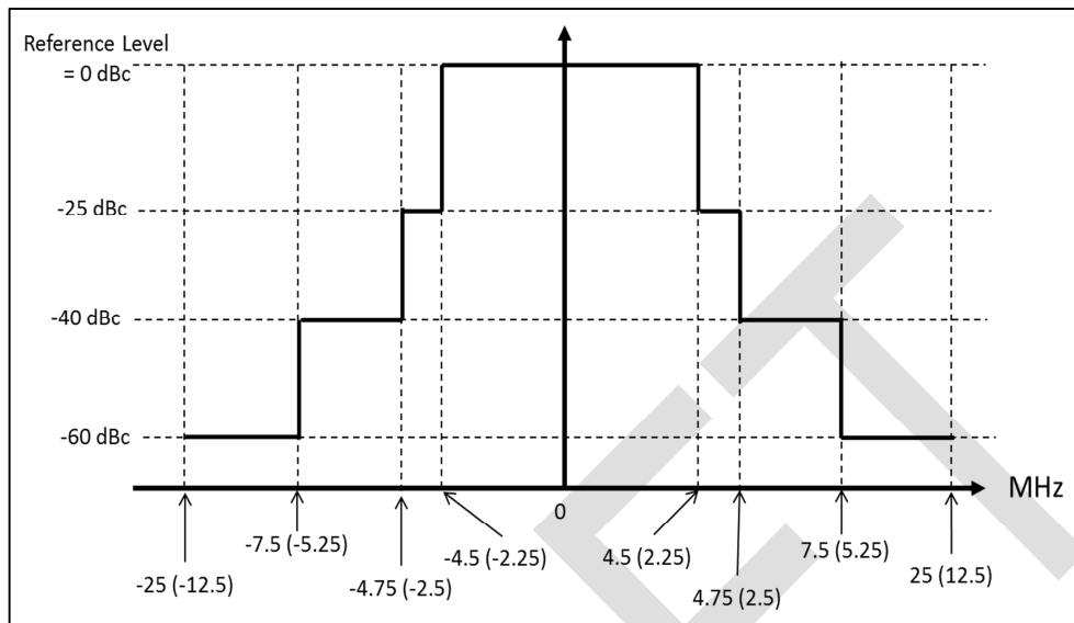
Figure 16: Spectral Emission Mask for both GS and AS
