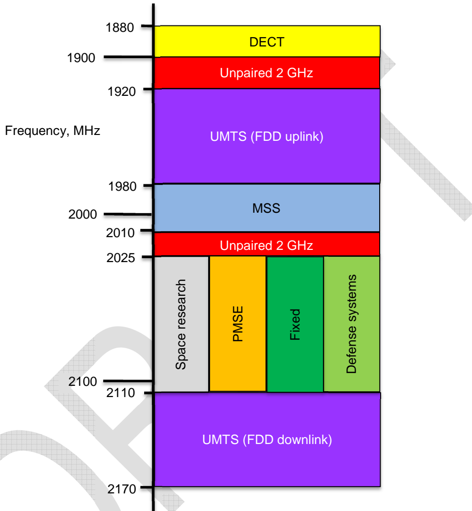
Figure 9: Adjacent band usage
