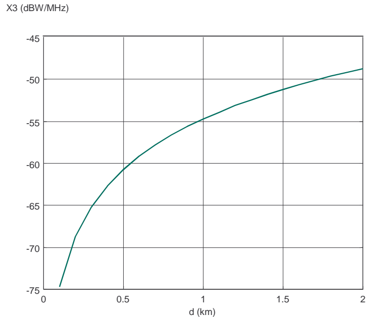
Figure 4: Required CS-to-CS spacing for un co-ordinated deployment
